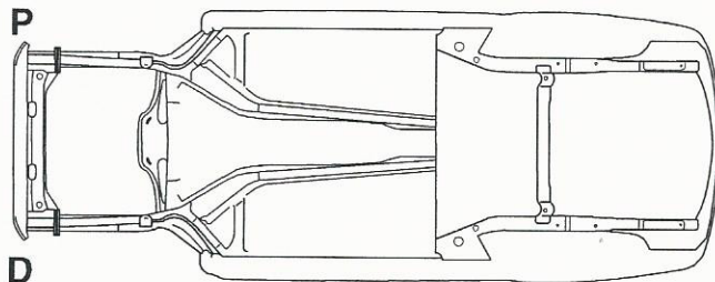
UNDERBODY VIEW
