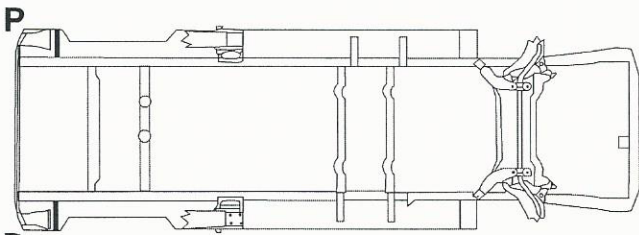
UNDERBODY VIEW
