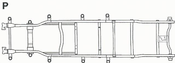
UNDERBODY VIEW
