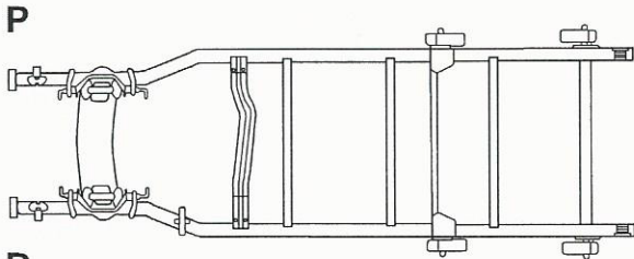
UNDERBODY VIEW
